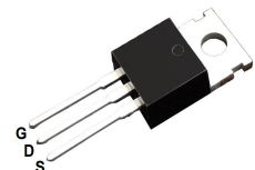
TO-220C
