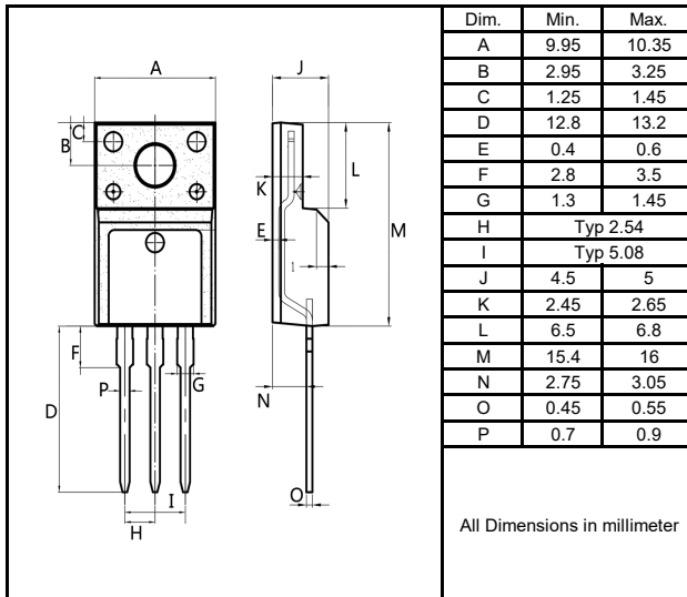
T0-220F
