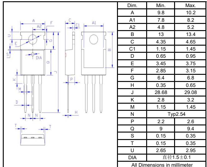
T0-220C
